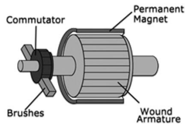
Brushed DC Motor
